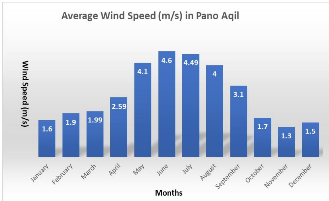
Figure 3.7: Graphical representation of average wind speed in Pano Aqil Cantt
