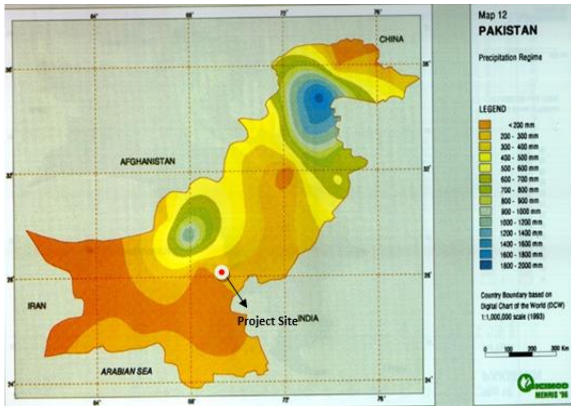
Figure 3.6: Precipitation Map of Pakistan
