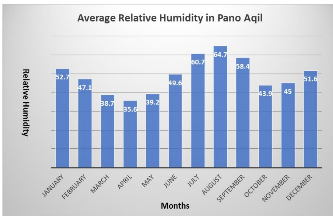
Figure 3.8: Graphical representation of average relative humidity in Pano Aqil Cantt
