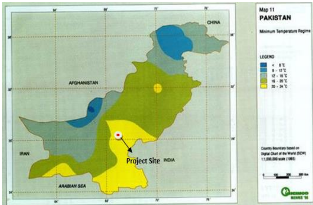
Figure 3.5: Minimum Temperature Regime Map of Pakistan
