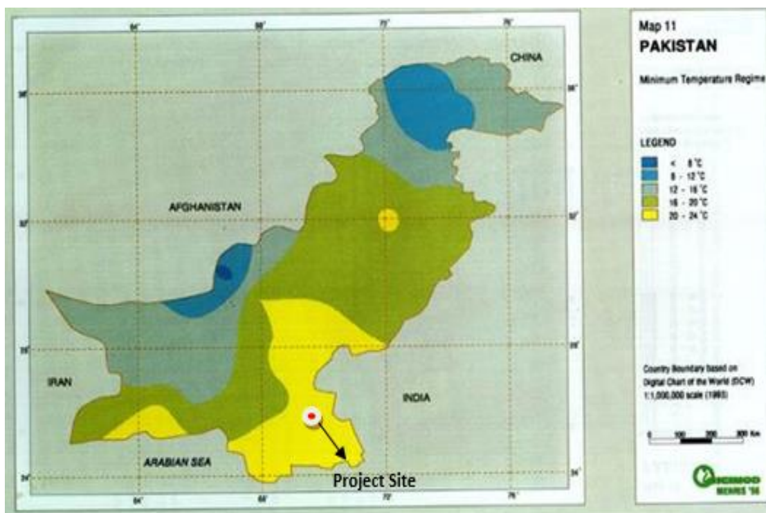
Figure 3.5: Minimum Temperature Regime Map of Pakistan
