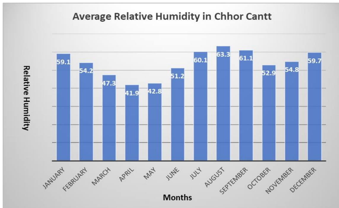
Figure 3.8: Graphical representation of average relative humidity in Chhor Cantt
