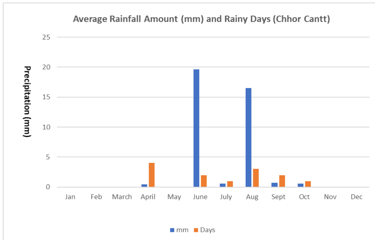
Figure 3.3: Graphical representation of Average Rainfall
