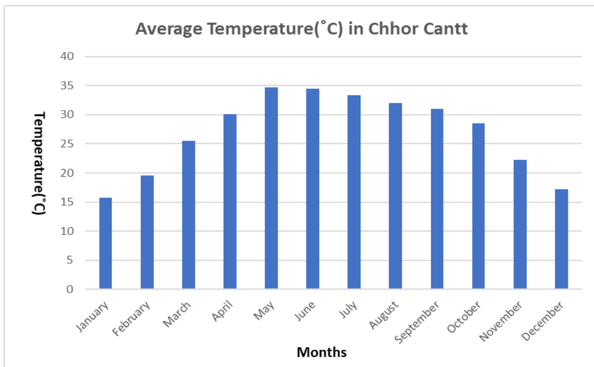
Figure 3.2: Graphical representation of Temperature
