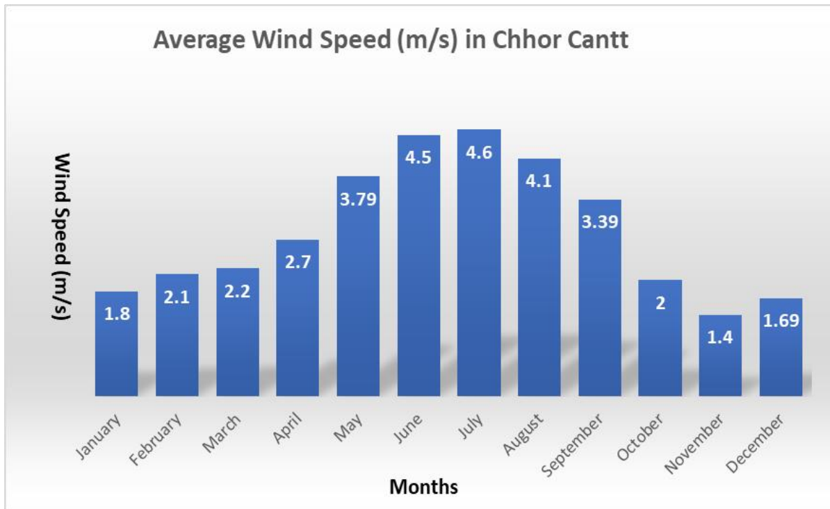
Figure 3.7: Graphical representation of average wind speed in Chhor Cantt
