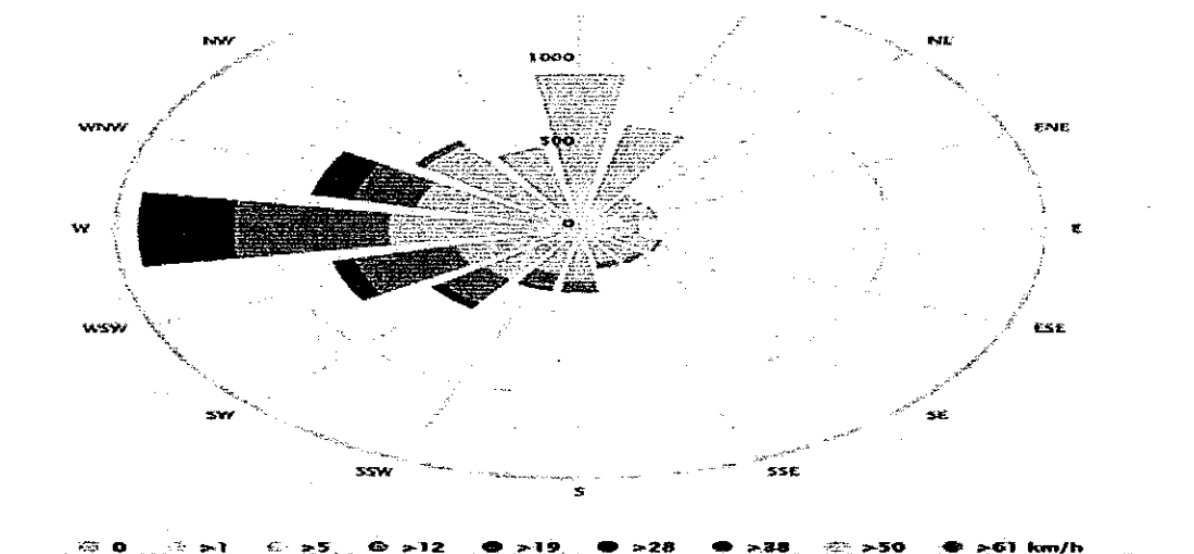
Figure 12 Wind Pattern in Quetta
