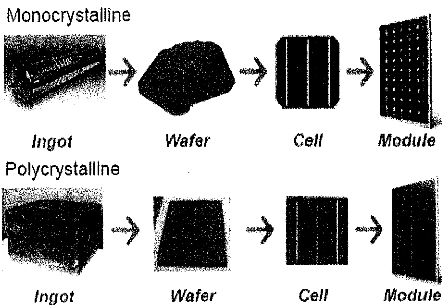
Figure 8: Solar panel Poly vs Mono
