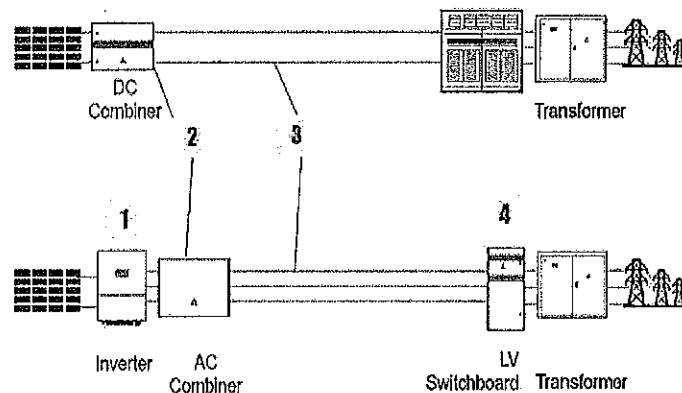
Figure 11: BoP comparison between Central and String inverters.
