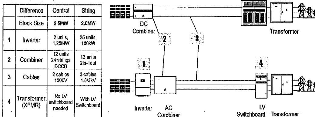
Figure 11: BoP comparison between Central and String inverters.
