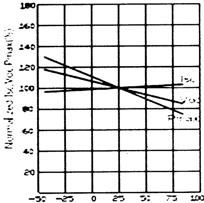
Temperature Dependence of Isc, Voc, Pmax
