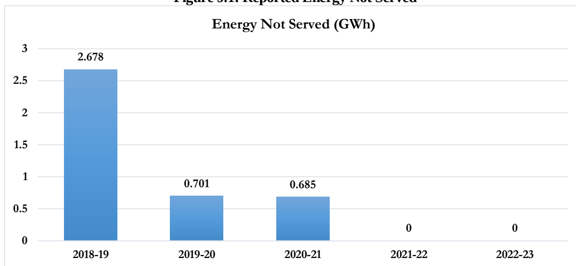
Figure 9.1: Reported Energy Not Served
