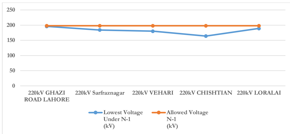
Figure 5.7: Lowest voltage (kV) recorded at 220 kV grid stations under N-1 condition
