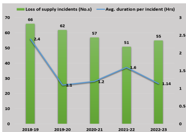
Figure 4.2: Loss of supply incidents & duration per incident
