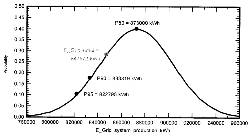
Probability distribution
