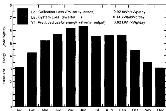
Normalized productions (per installed kWp): Nominal power 608 kWp
